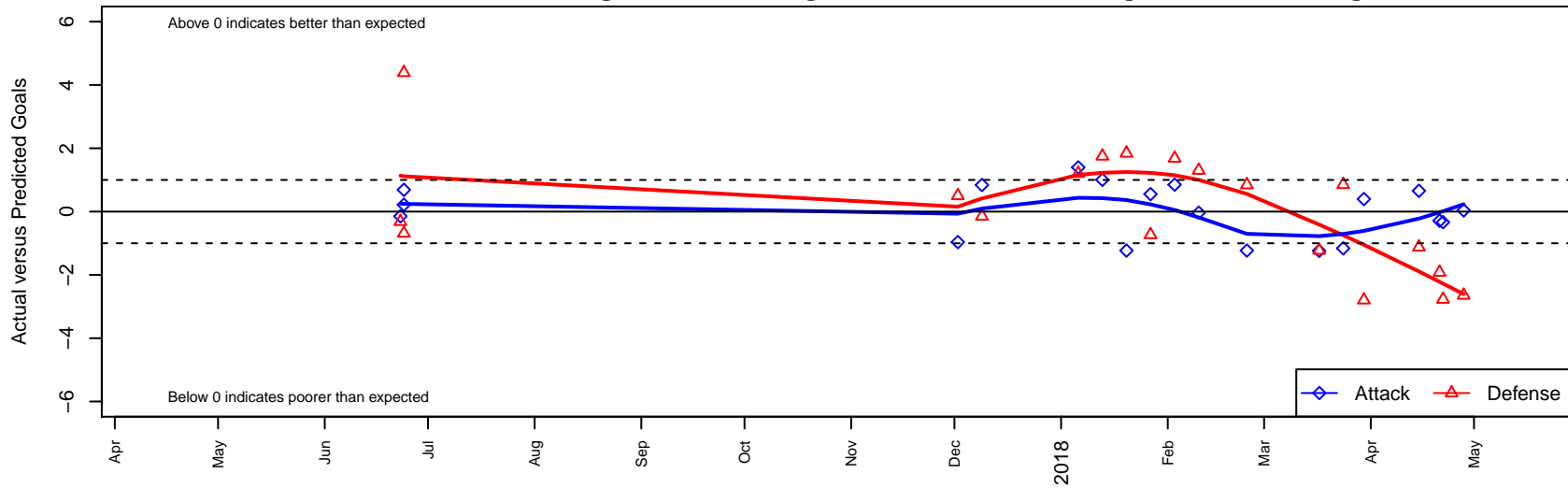
Irish FC Gators G02 Dots are actual minus expected GF (blue circles) and GA (red triangles). Blue line is smoothed change in attack strength. Red is smoothed change in defense strength.
